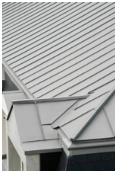
Clipped undercloak and overcloak
