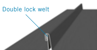
Double lock standing seam joint
