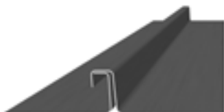
Small gap at base forms automatically and allows for lateral thermal expansion
