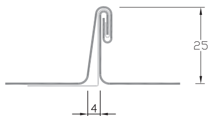
Double lock standing seam joint
